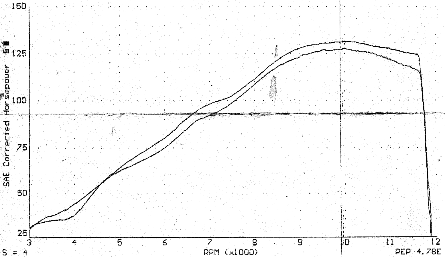
As measured on DYNOJET'S MODEL 150 DYNAMOMETER
